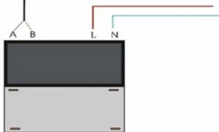
Air conditioning switch
