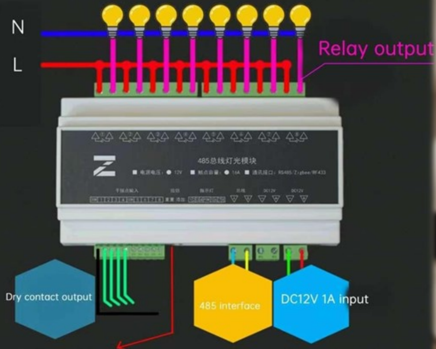
Load output wiring diagram
